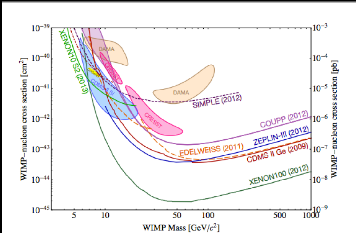
Figure 4-1. Constraints on spin-independent WIMP-nucleon cross sections as a function of WIMP mass
