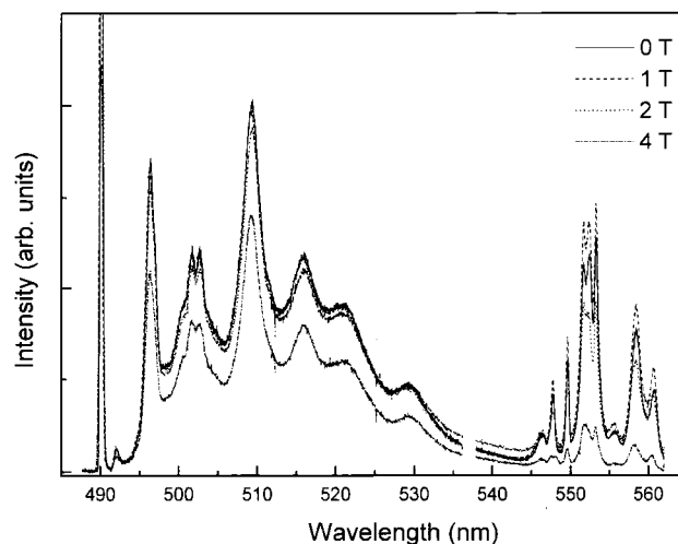
Fig. 2. Cooperative luminescence and up-conversion for several magnetic fields.
