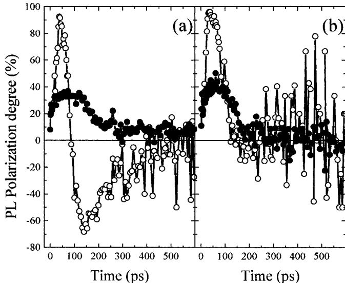
Fig. 3. a) Time evolution of the polarization degree of the cavity mode for 16 (●) and 40 W/cm 2 (○), in a point of the sample with a normal mode splitting of 4.5 meV. b) Time evolution of the polarization degree of the cavity mode for 25 (●) and 45 W/cm 2 (○), for a normal mode splitting of 6 meV
