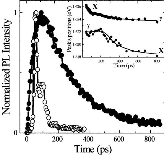
Fig. 2. Time evolution of the cavity mode for excitation densities below ( 9 \text{ W/cm}^2 , ●) and above ( 25 \text{ W/cm}^2 , ○) the threshold for stimulated emission. Inset: Energies of both polariton branches as a function of time. The lines are guides to the eye
