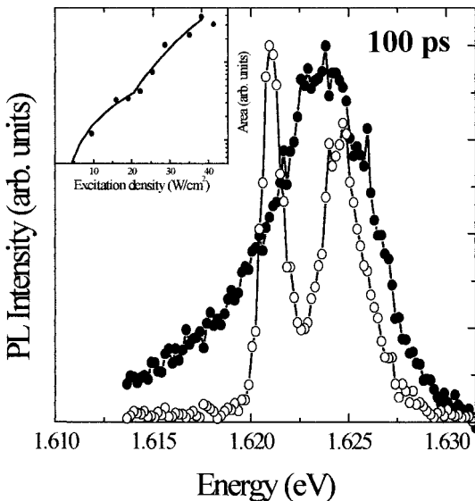
Fig. 1. Time-resolved PL spectra taken 100 ps after excitation, for excitation densities below ( 9 \text{ W/cm}^2 , \bullet ) and above ( 25 \text{ W/cm}^2 , \circ ) the threshold for stimulated emission. Inset: Integrated emission (in logarithmic scale) of the LPB at 100 ps versus excitation density
