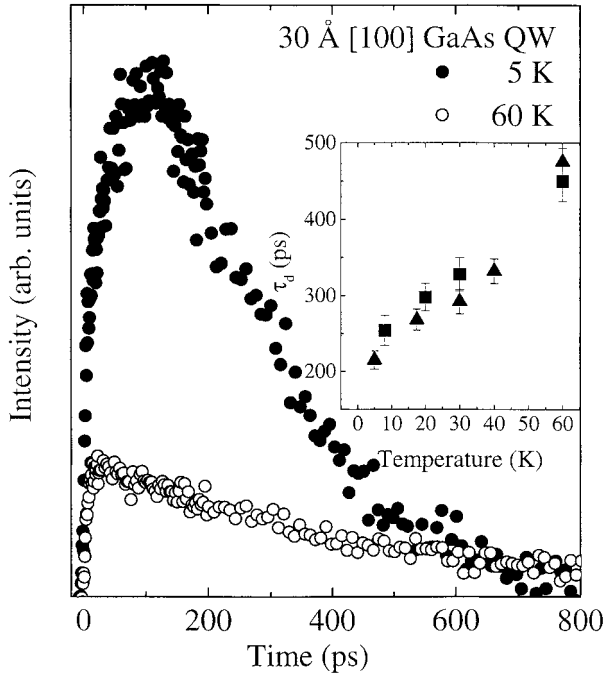
Fig. 2. Time evolution of the PL for two different temperatures: 5 K (solid circles) and 60 K (open circles). The inset shows the temperature dependence of the decay time obtained from time traces (triangles), and from fits of decay of the integrated emission band (squares)
