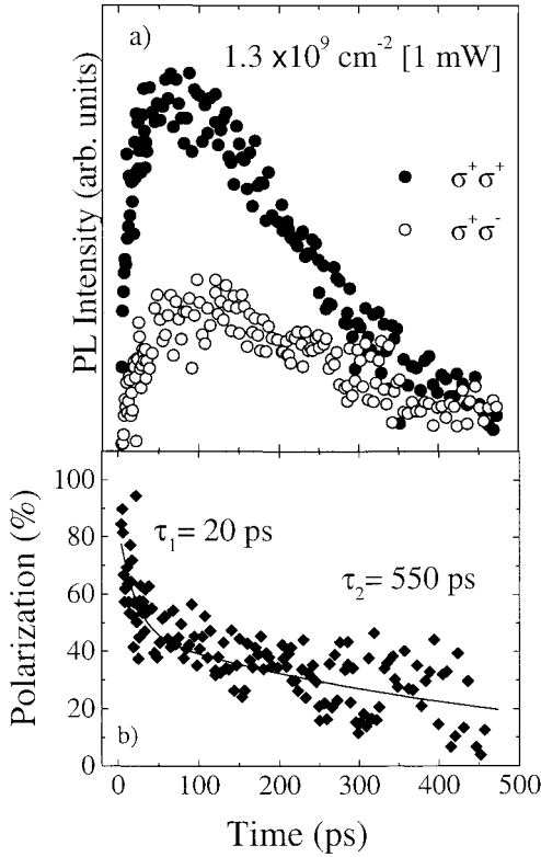
Fig. 3. a) Time evolution of the PL exciting with \sigma^+ polarized pulses at 1.717 eV: \sigma^+ (solid circles) and \sigma^- (open circles) polarized emission. b) Time evolution of the polarization degree; the line is the best fit to a double-exponential decay
