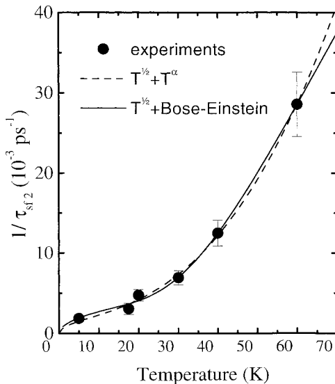
Fig. 4. Temperature dependence of the “electron” spin-flip rate. The lines represent the best fit to the predictions of Dyakonov-Perel and exchange mechanisms (dashed) or Dyakonov-Perel and scattering by phonons (solid)
