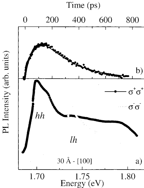
Fig. 1. a) Photoluminescence excitation spectra for the 30 Å thick QW grown on a [100] GaAs substrate under \sigma^+ excitation: \sigma^+ (black dots) and \sigma^- (gray dots) polarized emission. b) Time evolution of the unpolarized photoluminescence exciting at 1.717 eV and detecting at the PL peak; the line is the best fit to a three level model (see text)
