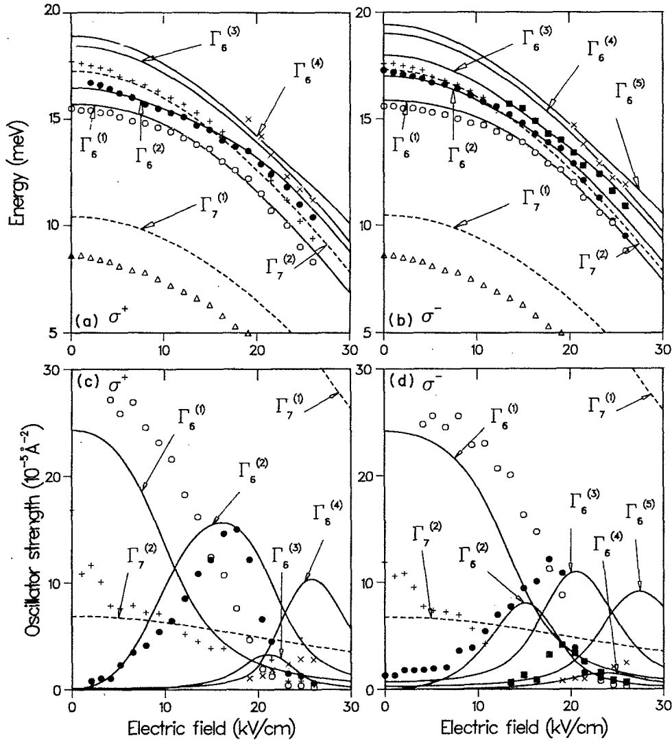
FIG. 2. Energy shifts, (a) and (b), of excitons in a 160-Å quantum well as a function of electric field normal to the well, for \sigma^+ and \sigma^- polarizations, respectively. A magnetic field of 0.5 T was applied parallel to the electric field. Oscillator strengths, (c) and (d), corresponding to (a) and (b), respectively. The lines represent the results of the calculations. See Table I for the labeling of the states.
