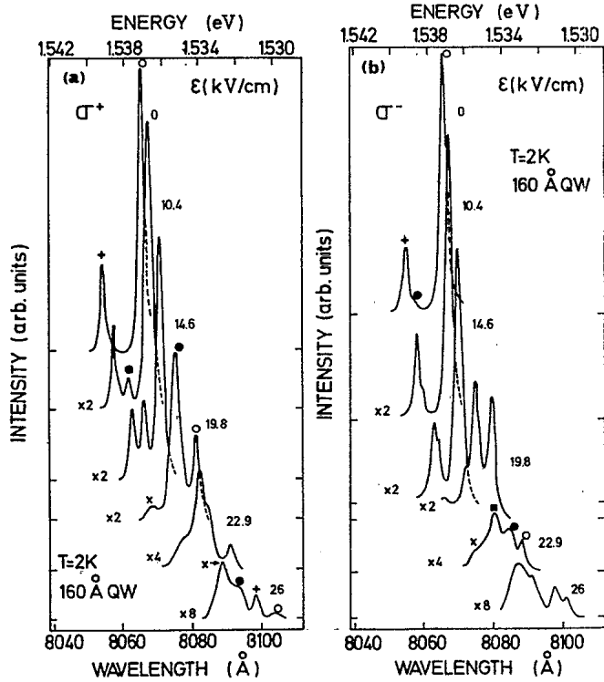
FIG. 1. Low-temperature photoluminescence excitation spectra of a 160-Å quantum well at several electric fields normal to the well. The excitation was performed with \sigma^+ and \sigma^- polarizations in (a) and (b), respectively. Scaling factors are indicated on the left-hand side of the spectra. A magnetic field of 0.5 T was applied parallel to the electric field.
