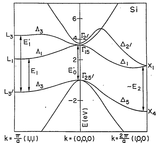
FIG. 1. Band structure of Si calculated within the k \cdot p method (from Ref. 3), showing the main interband critical points.
