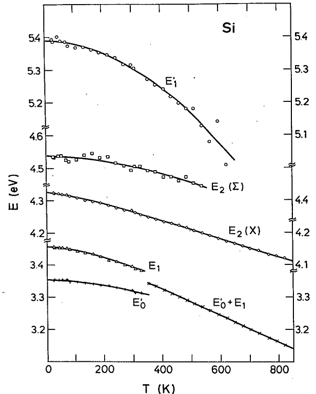
FIG. 6. Temperature dependence of the interband critical point energies of Si. The solid lines represent the best fits with Eqs. (3). The function used and the values of the parameters involved are given in Table I.
