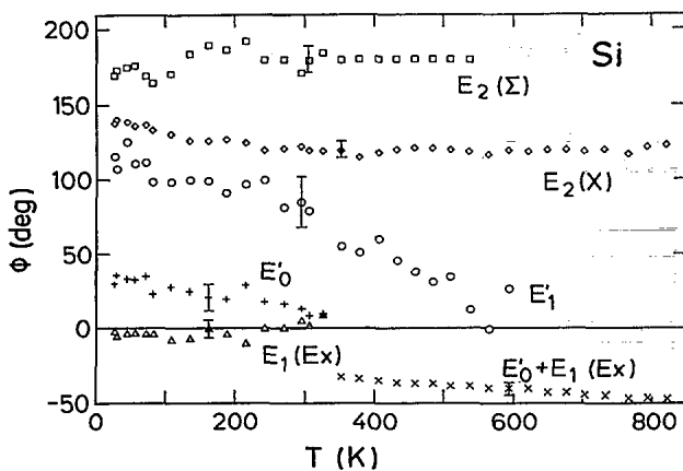
FIG. 8. Temperature dependence of the phase angle \Phi , defined in Eq. (2), measured for the interband CP's of Si.
